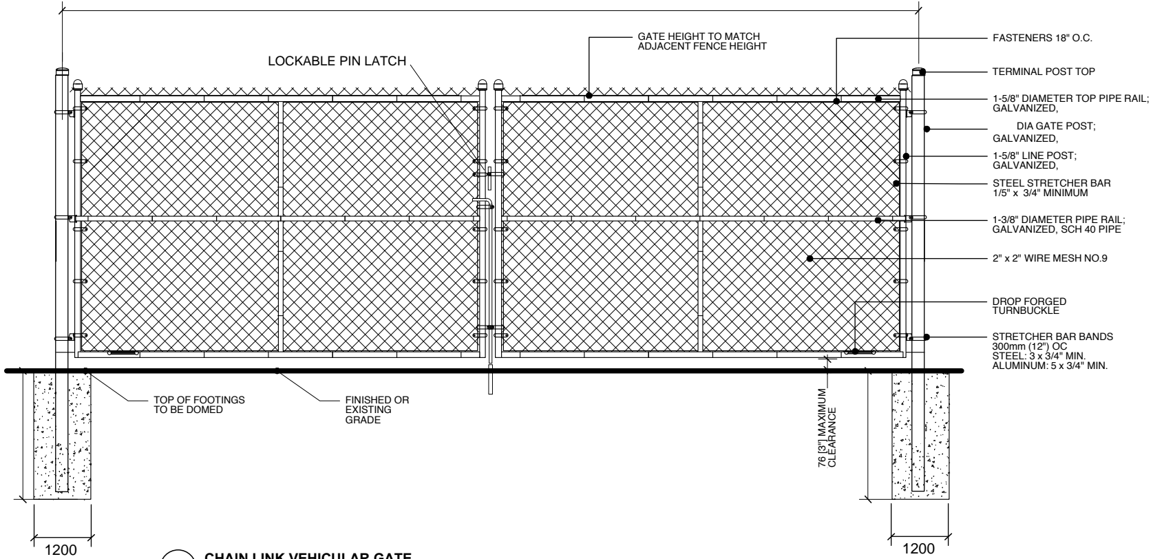
9 CHAIN LINK VEHICULAR GATE
