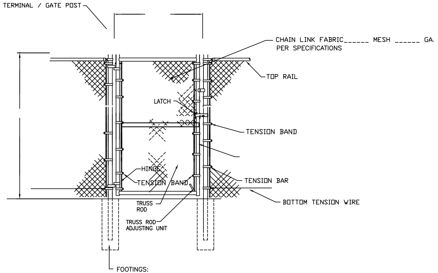
GATE PLAN
